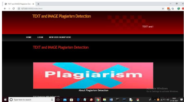
Fig.4 Home Page
